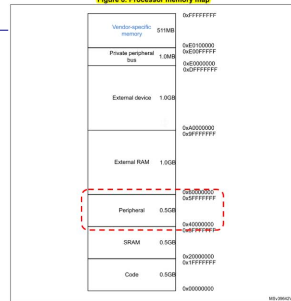
Figure 8. Processor memory map
