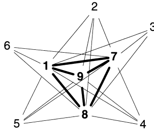
Fig. 3. Core/periphery structure.
