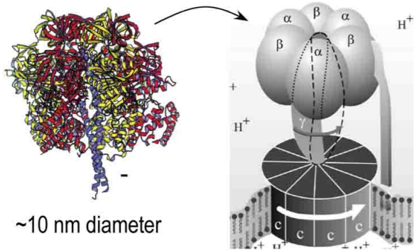
ATP synthase
