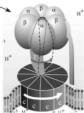
ATP synthase
