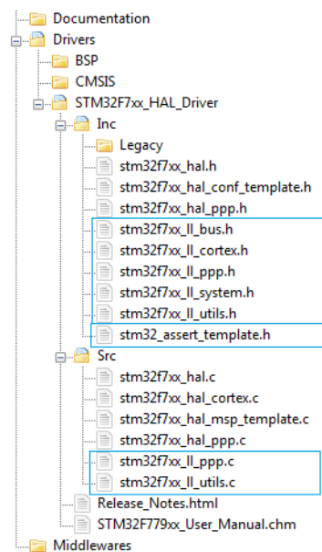
Figure 8. Low-layer driver folders
